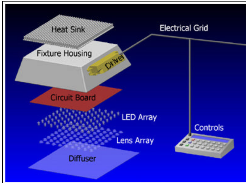
Figure 6. LED lighting system anatomy.
