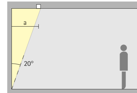
To achieve an even light distribution on the wall, the offset (a) of the luminaire from the wall should be at least one third of the room height.
