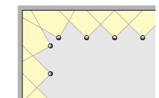
The side striation produced by the above-mentioned arrangement can be avoided by having a double wallwasher arrangement in the corner.
