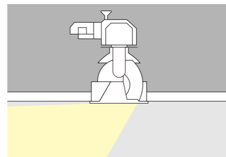
The double-focus wallwashers achieve an excellent uniformity on the wall due to the design of their reflectors. By completely concealing the lamp using an anti-dazzle cone the design simultaneously ensures exceptional visual comfort.
