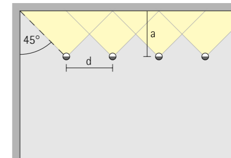
A wallwasher in a room corner should be positioned on the 45° line between the two walls. The brightness can then fade unnoticeably towards the corner and can also remain inconspicuous on the side wall.
